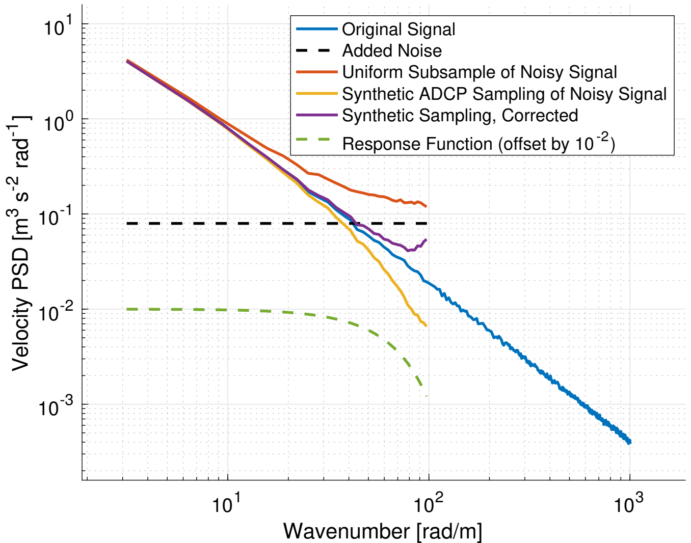
FIG. 2. Synthetic data created to have a power spectrum of the form k^{-5/3} was sampled with a uniform sub-sample (orange), and with a double rectangular filter that mimics the sampling from an ADCP (yellow). White noise is added during both of the synthetic sampling procedures (dashed black), and the power spectrum of the sampled synthetic data is compared with the spectrum from the original synthetic time series (blue). The corrected, synthetically sampled spectrum (purple) fits the original signal over a much larger wavenumber range. The convolution filter described in Equation 6, is shown in dashed green, offset for clarity.
