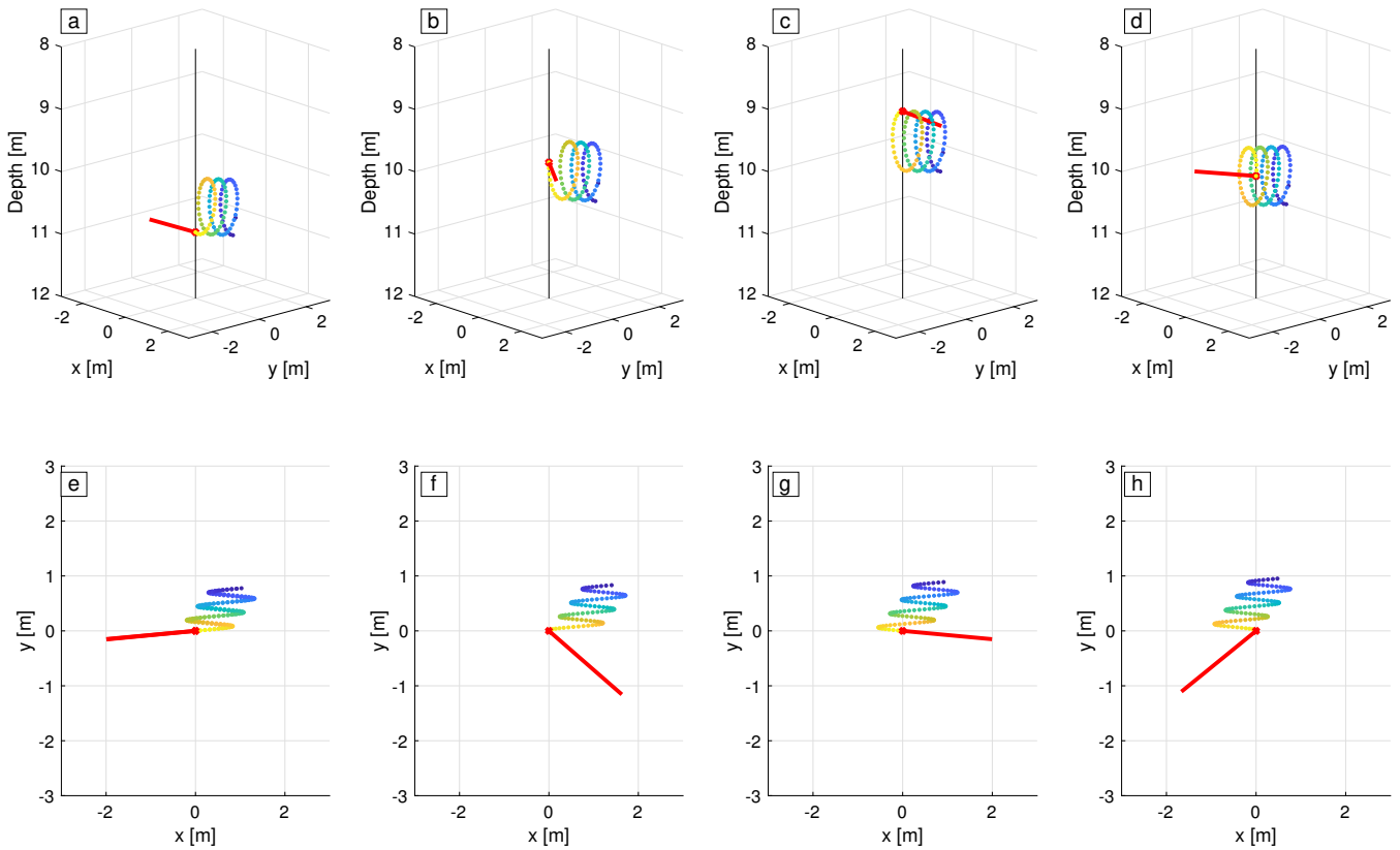
FIG. 15. Here, panels show four phases of a simulated wake with monochromatic waves and a constant off-wave angled mean velocity. The top panels (a-d) show snapshots of the 3D view of the wake at four unique phases. The bottom panels (e-h) show a top-down 2D view during the same phases as above (a-d). The red line shows the up-flow direction mimicking the expected orientation of the ADCP. The yellow-to-blue circles show a simulated wake, with locations determined through the advection of the previous instrument locations. The simulated wake's color scale indicates timing of wake creating. The vertical line in (a-d) shows a reference mooring line. Here, simulated 8s-period 2m-in-height monochromatic waves propagate in the positive x direction, with a small mean cross-flow ( U_y/U^{orb} = 0.075 , U_y = 0.03 \text{ m s}^{-1} ) in the positive y direction. At no part of the wave period does the simulated ADCP beam intersect the wake.
