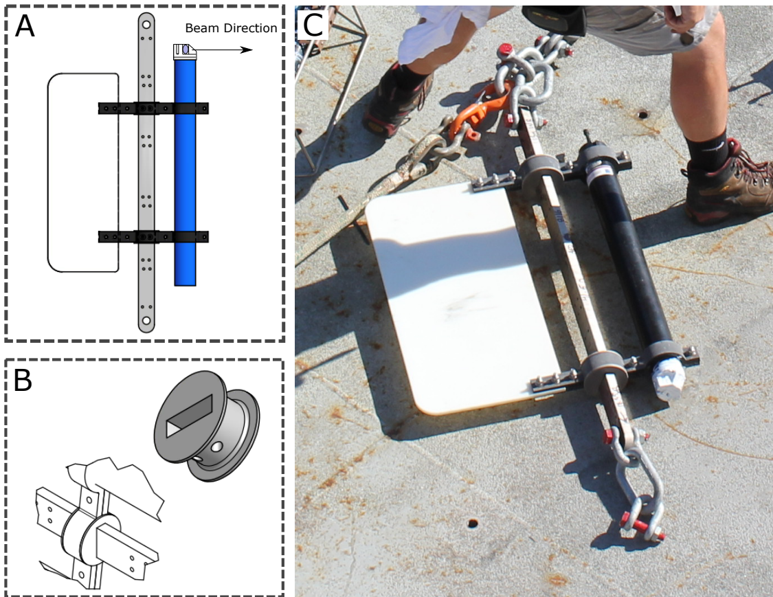
FIG. 4. A side-on view of the Aquadopp mount showing the no-weld titanium bar, Delrin clamps, and orientation fin is shown in panel A. Panel B shows the Delrin-Delrin swivel that attaches the ADCP clamp to the titanium bar. A picture of the configured mount on deck before deployment as part of the SPURS-2 mooring is shown in panel C. The Aquadopp is equipped with the current meter transducer head, with the active beam oriented in the horizontal plane pointing up-flow from the directional fin.
