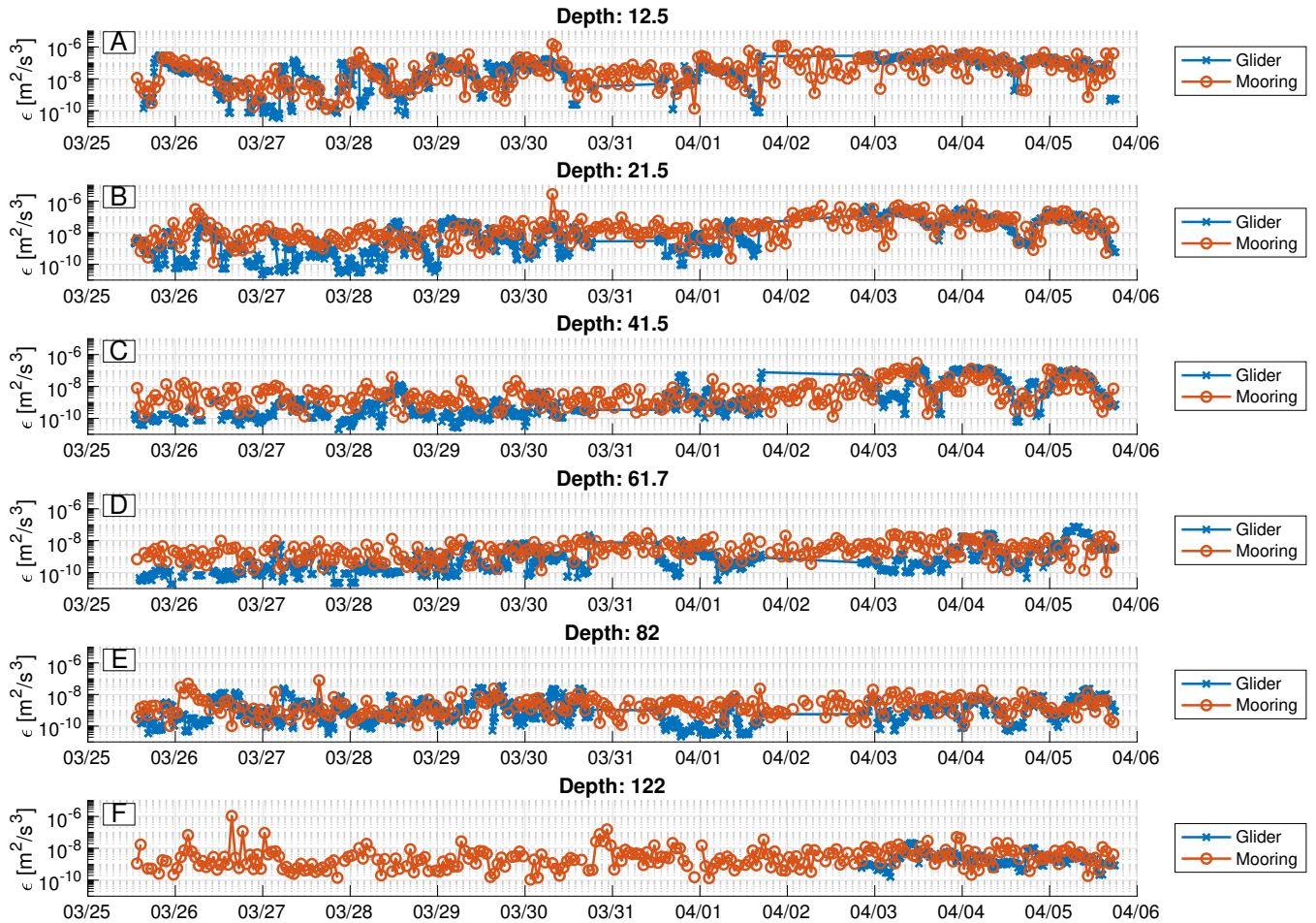
FIG. 10. Comparison of time-smoothed glider-derived microstructure dissipation rates and mooring-derived dissipation rates for all depths during the second glider deployment in March and April of 2013. Measurements at depths of 12.5 m, 21.5 m, 41.5 m, 82 m, and 122 m, were made by 2 MHz instruments, with measurements at 61.7 m made by a 1 MHz instrument. Agreement between the glider and mooring measurements is best during the dates of April 3rd to April 6th.
