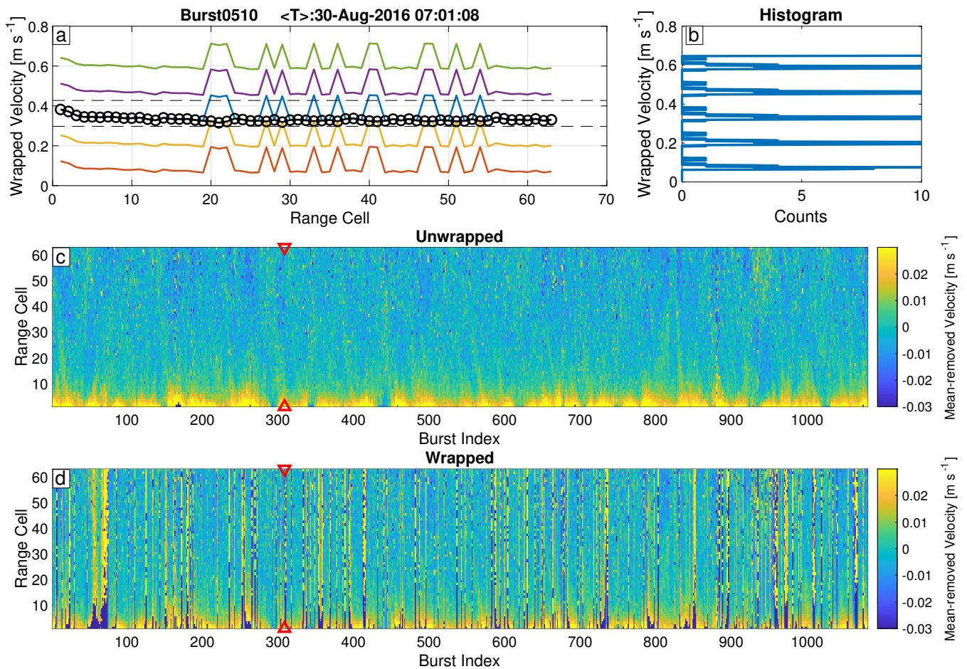
FIG. 5. An example of the unwrapping procedure shown for an arbitrary burst (SPURS-2, 41.5m Depth). Panel (a) shows an example of a wrapped profile that has been multiplied by 2nV_r . The unwrapped profile is shown with the black circles. The histogram used to find the groupings of unwrapped data is shown in panel (b). Panel (c) shows the mean-removed unwrapped velocities for the entire burst, consisting of 1080 profiles. The mean-removed wrapped data is shown in panel (d) for comparison. Red triangles mark the specific profile shown in (a) and (b).
