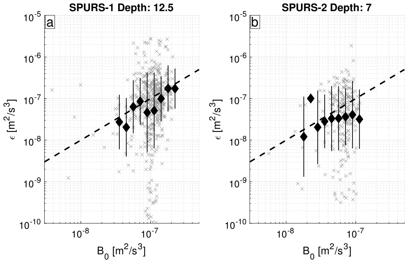
FIG. 12. Upper SPURS-1 (a) and SPURS-2 (b) dissipation rate estimates compared to surface buoyancy flux (COARE) during strong convective conditions z/L < -5 , and above the mixed-layer depth z/MLD < 0.75 . Data arbitrarily binned with 35 even intervals in log space between 10^{-9} to 10^{-6} are shown in solid black diamonds with vertical bars showing one standard deviation within the bin. Bin averages are only shown if they contain more than 10 data points.
