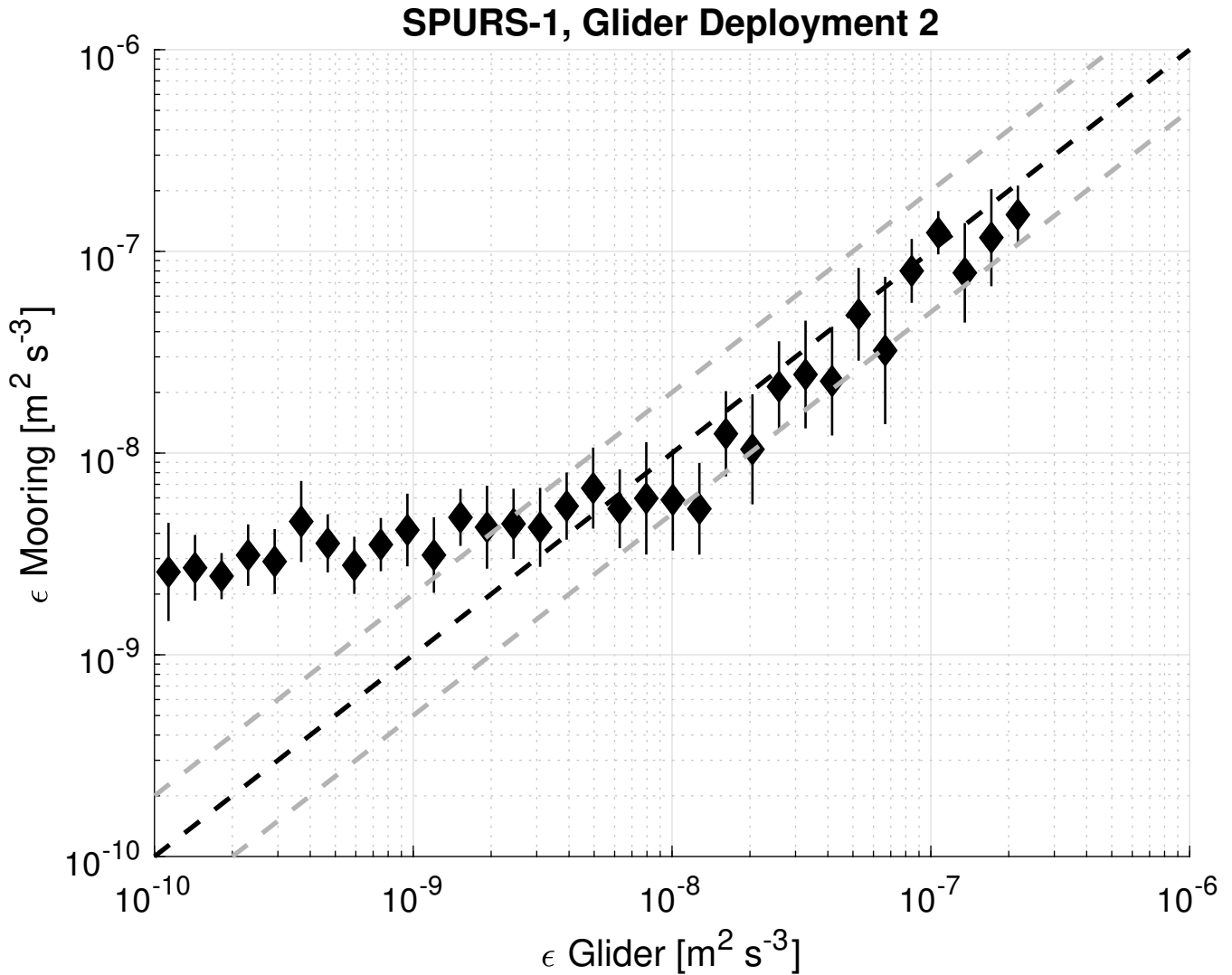
FIG. 11. Direct comparison of time-smoothed microstructure dissipation rates and mooring-derived dissipation rates for all depths (12.5, 21.5, 41.5, 61.7, 82, 122) during the second glider deployment in March and April of 2013. The vertical bars show the 95% confidence interval of the log-mean (1.96 times the standard error). Bin averages with less than 10 values are excluded, and bins were arbitrarily chosen as 40 evenly log-spaced bins on the interval 10^{-10} to 10^{-6} . Dashed black line shows the 1:1 agreement level. As in Figure 9, agreement between the two dissipation rate estimates is good above \epsilon = 10^{-8} \text{ m}^2 \text{ s}^{-3} .
