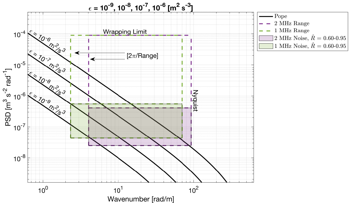
FIG. 3. Example one-sided turbulence spectra for dissipation rates \epsilon = 10^{-9}, 10^{-8}, 10^{-7}, 10^{-6} \text{ m}^2 \text{ s}^{-3} are shown for both the Pope model spectrum (black). The overlaid dashed boxes show the range of wavenumbers sampled, the maximum spectral estimates due to phase wrapping (Equation 9) and the range of white noise levels predicted by Equation 7 bounded by the minimum mean along-beam correlations allowed in quality control (see Section 2.d.2), and the (roughly) highest returned correlation level ( \hat{R} = 0.6 , and \hat{R} = 0.95 , shaded boxes). We note that these noise levels are not guaranteed, and that it is possible a mix of different instrument configurations and environmental variables could result in uniformly lower correlations (and thus noise levels). The values here are representative of observed noise levels across multiple mooring deployments used in this study. The color of the dashed box differentiate the 1 MHz (green) and 2 MHz (purple) instruments. Based on this parameter space, we expect to resolve the inertial subrange for \epsilon \sim 10^{-8} - 10^{-5.5} \text{ m}^2 \text{ s}^{-3} , with measurement of dissipation rate \epsilon \sim 10^{-9} - 10^{-8} \text{ m}^2 \text{ s}^{-3} possible with high correlation returns.
