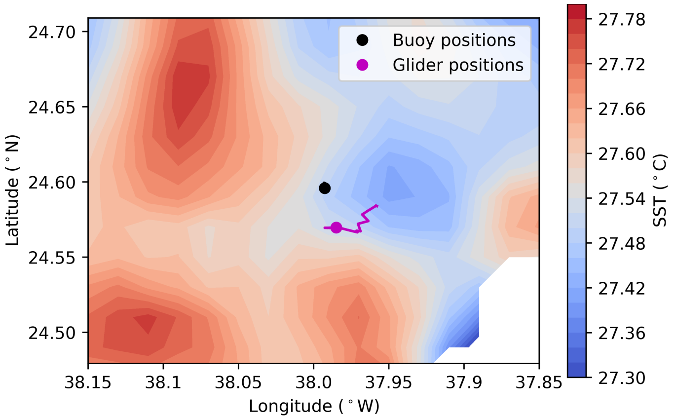
FIG. 14. Satellite derived SST taken on 9/30/2012 at 03:30:02 is shown with positions of the SPURS-1 central mooring and the glider track during the September-October sampling period (i.e., data shown in Fig. 8). SST variability on the order of 0.2\text{ }^{\circ}\text{C} exists over small scales, suggesting some of the differences in local water properties and turbulent statistics seen between the mooring and glider data sets are physical rather than manifestations of sensor or methodology errors.
