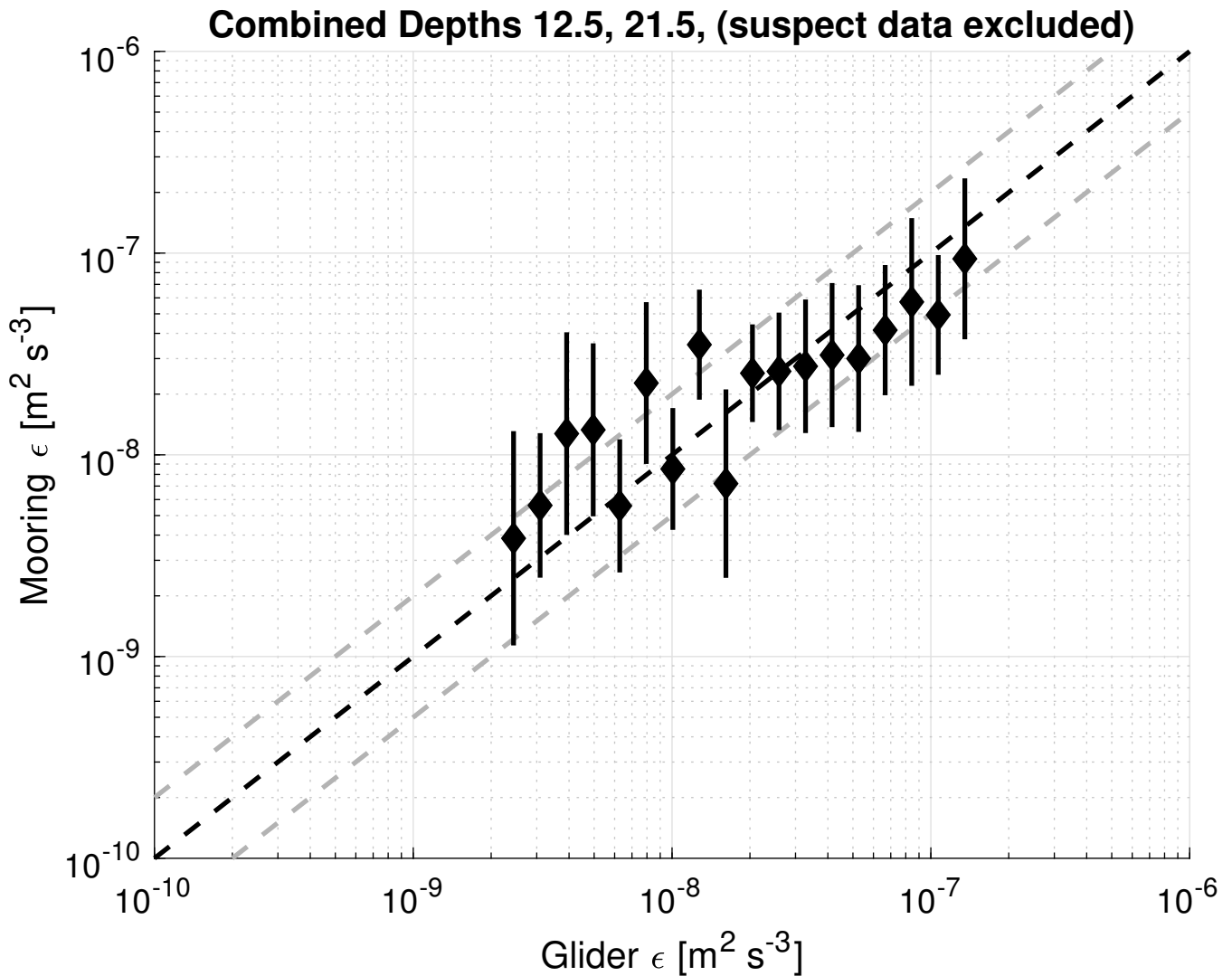
FIG. 9. Direct comparison of time-smoothed microstructure dissipation rates and mooring-derived dissipation rates for both 12.5 m and 21.5 m depths. Boxed regions in Figure 8 have been excluded. Black diamonds represent log-mean bin averages, with associated vertical bars showing the 95% confidence interval of the log-mean (1.96 times the standard error). Bin averages with less than 10 values are excluded, and bins were arbitrarily chosen as 40 evenly log-spaced bins on the interval 10^{-10} to 10^{-6} \text{ m}^2 \text{ s}^{-3} . Dashed black line shows the 1:1 agreement level. Mooring and glider derived dissipation rates agree well above \epsilon of \sim 10^{-8} \text{ m}^2 \text{ s}^{-3} , below which the mooring-derived estimates appear biased. Confidence in the mean is roughly a factor of 2 (gray dashed lines), similar to previous studies (Moum et al. 1995).
