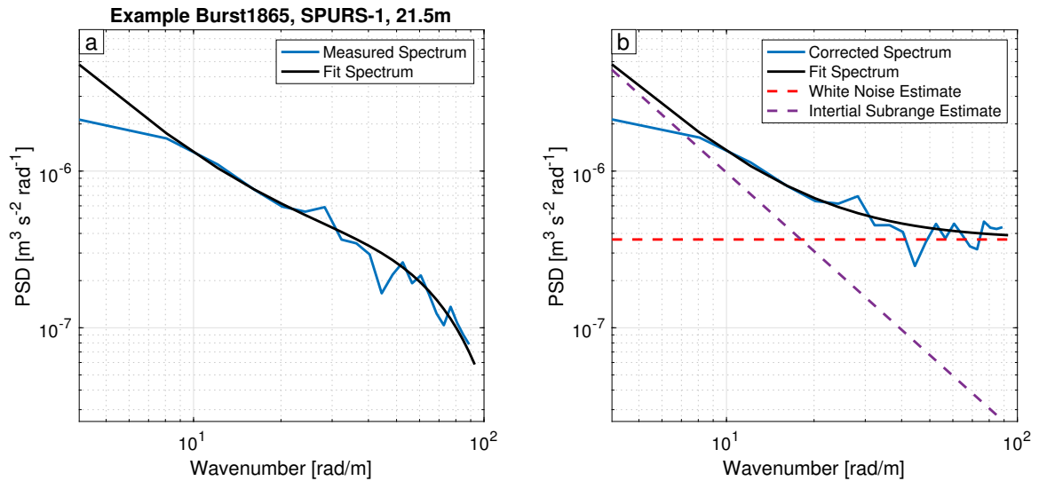
FIG. 7. An example of a spectral fit is shown. (Left) The fit includes the sampling filter (e.g., Fig. 2. and Equation 6), resulting in the high-wavenumber roll-off despite the existence of white noise. (Right) The measured spectrum and fit are corrected for the effect of the sampling filter, and shown with the components of the best fit model, where the estimated white noise level is shown with the dashed red line, and the estimated inertial subrange level is shown with the dashed purple line. The sum of the dashed lines is equal to the solid black best-fit determined through regression.
