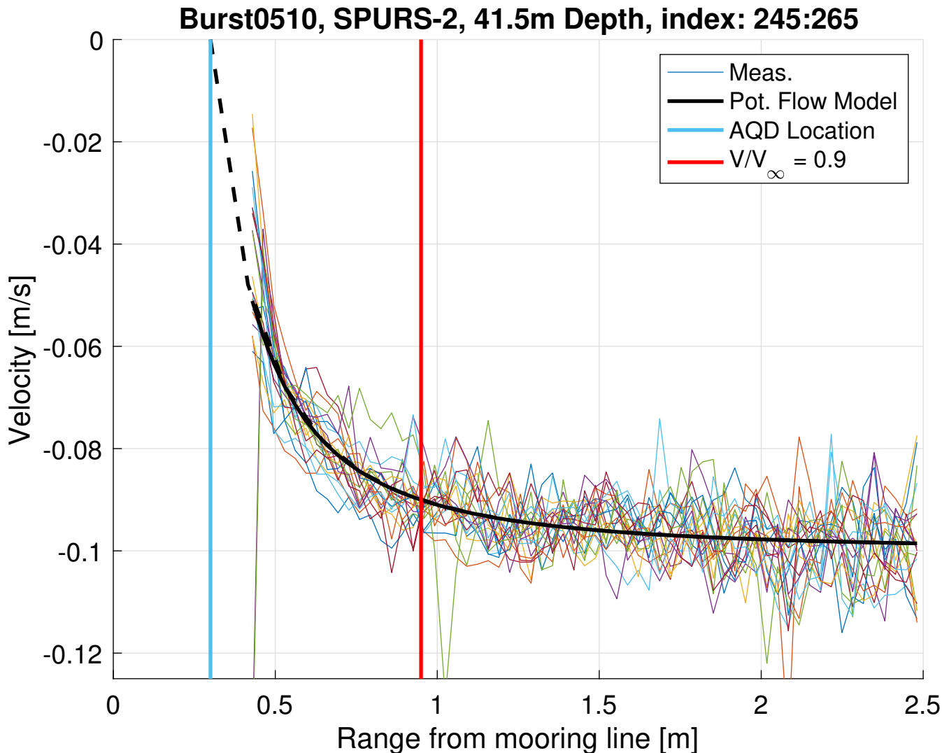
FIG. 6. Example velocity profiles shown in distance from mooring line (thin colors). The potential flow solution for flow around a cylinder with radius of 0.3 m and V_{\infty} = 0.1 is shown in black. The vertical blue line shows the location of the Aquadopp head, 30 cm from the mooring line (equivalent to the estimated cylinder radius), and a vertical red line shows the range where the potential flow is 90% of the free stream velocity, nearly 1 m from the mooring line, and 63 cm from the Aquadopp head. The measured velocity profiles have ambiguous absolute velocity values, but are shown here offset by the assumed V_{\infty} value.
