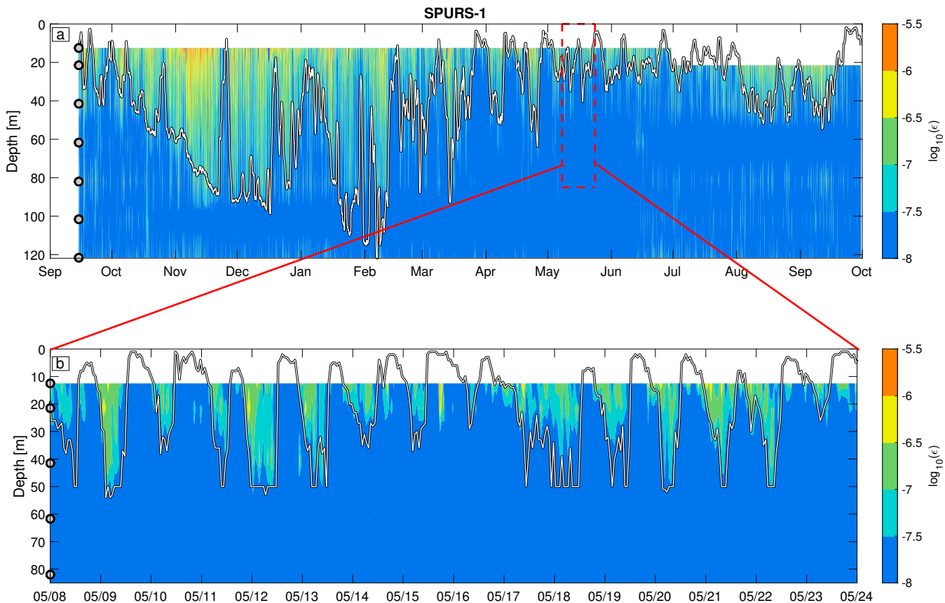
FIG. 13. Contour plots are shown of TKE dissipation rate estimates for SPURS-1 with the depth of the estimates shown with grey circles to the left. Hourly estimates of mixed layer depth are shown above the contours (estimated as the depth at which temperature is 0.05^{\circ}\text{C} different from the surface value), with (a) showing 24 hour moving mean for clarity. The full duration results are shown in (a), and generally show dissipation rates are larger above the temperature-estimated mixed layer depth. Panel (b) shows diurnal variability in TKE dissipation rates are consistent with the variability in the mixed-layer depth. Missing values have been interpolated in both panels.
